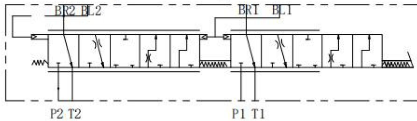
hydraulic symbol
